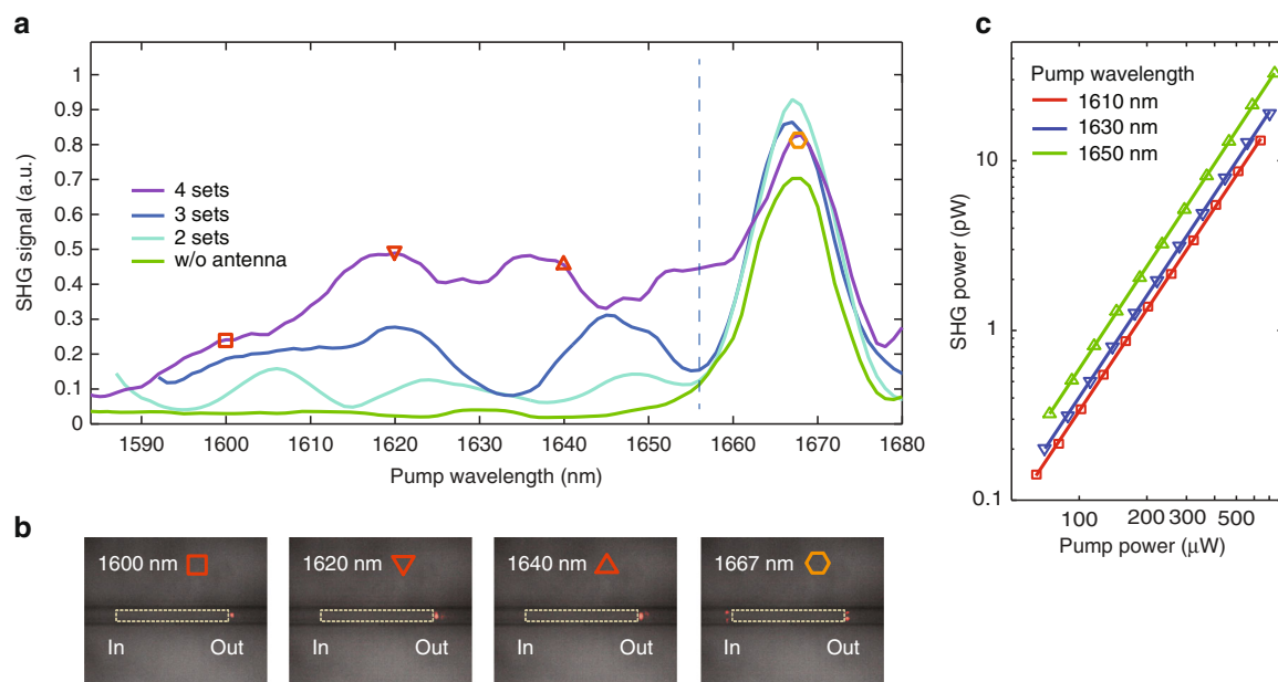
Fig. 4 Experimental results. a Measured SHG power at the output port of devices patterned with different number of phased antenna arrays, in comparison with that of a bare LiNbO 3 waveguide, showing broadband SHG enhancement (to the left of the dashed line). The narrow SHG peak at a pump wavelength of 1667 nm (to the right of the dashed line), which exists in all tested devices including bare LiNbO 3 waveguides, is the result of an accidental phase-matching between the pump, TE 00 ( \omega ), and the seventh-order TE waveguide mode at the SH frequency, TE 06 (2 \omega ). b Top-view camera images showing the scattered SH light from a device patterned with a gradient metasurface consisting of four phased antenna arrays (indicated by the white dashed frames). At pump wavelengths of 1600, 1620, and 1640 nm, SH signal (red spots) is only observed at the output end of the gradient metasurface, which indicates that the SH signal is generated within the metasurface-covered section of the device. In contrast, at the accidental phase-matching peak wavelength of 1667 nm, scattered SH light appears at both the input and output ends, which indicates that the SH signal has already been generated by the phase-matching process before it enters the metasurface section. c Input-output power relations for the device showing quadratic power dependence between the pump and the SH signal at three different pump wavelengths
