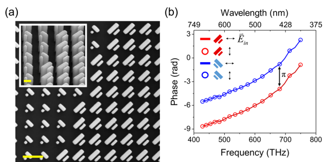
Figure 2. Implementation of metacorrector. (a) Scanning microscope image from a region of the metacorrector, made of TiO 2 nanofins on a glass substrate. Scale bar: 500 nm. The inset shows an oblique view (scale bar: 200 nm). Note that each element is aligned along either 45^\circ or -45^\circ , rendering the phase profile of the metacorrector the same for x and y polarizations. (b) Simulated phase shift of the transmitted electric field, which is orthogonal to the polarization of the incident light (eq 7). The incident polarization is oriented along the x or y axes (depicted by black arrows in the legend). To illustrate the principle, we simulated an element consisting of two nanofins with various rotation angles subjected to illumination with different polarization states. Note that a 90^\circ rotation introduces a \pi phase shift without changing the dispersion, and the element shows identical phase under x - and y -polarized light rendering the metacorrector capable of correcting aberrations for any incident polarization. The nanofin parameters ( w_1, l_1, w_2, l_2, g ) equal 90, 420, 70, 200, and 60, respectively, in nanometer units.
