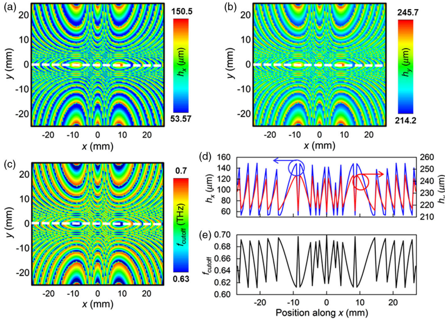
FIG. 5 Hollow dimensions of the designed ENZ GRIN lens: (a) contour plot showing the value of h_x as a function of the waveguide position ( x , y ). (b) Idem for h_y . (c) Cutoff frequency of the fundamental mode for all the waveguides. Hollow dimensions (d) and cutoff frequency for the waveguides located along the x axis at y = 0 . These values are obtained from the white dashed line of panels (a)–(c).
