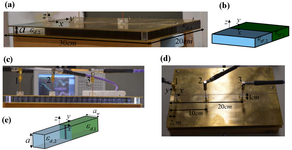
Figure 1. (a) Photograph of the parallel-plate-metamaterial waveguide filled with two dielectrics with positive permittivities, \epsilon_{d,1} and \epsilon_{d,2} . The distance between the metallic plates is a . (b) Effective medium model of the structure: two materials with equivalent permittivities, \epsilon_{ef,1} and \epsilon_{ef,2} , are separated by a planar interface. (c) Front view of our structure, showing the thin metallic wires that suppress the excitation of TM modes at the interface. (d) Top view of the structure. The dipole antennas are inserted at a distance x = 2 cm, x = 10 cm and x = 20 cm from the sidewall. (e) Unit cell of the equivalent periodic structure formed by two half-spaces filled by materials with permittivities, \epsilon_{d,1} and \epsilon_{d,2} , and a single wire at the interface (the top and bottom metallic walls are not shown). The period of the structure along the x -direction is a_w = 3 mm.
