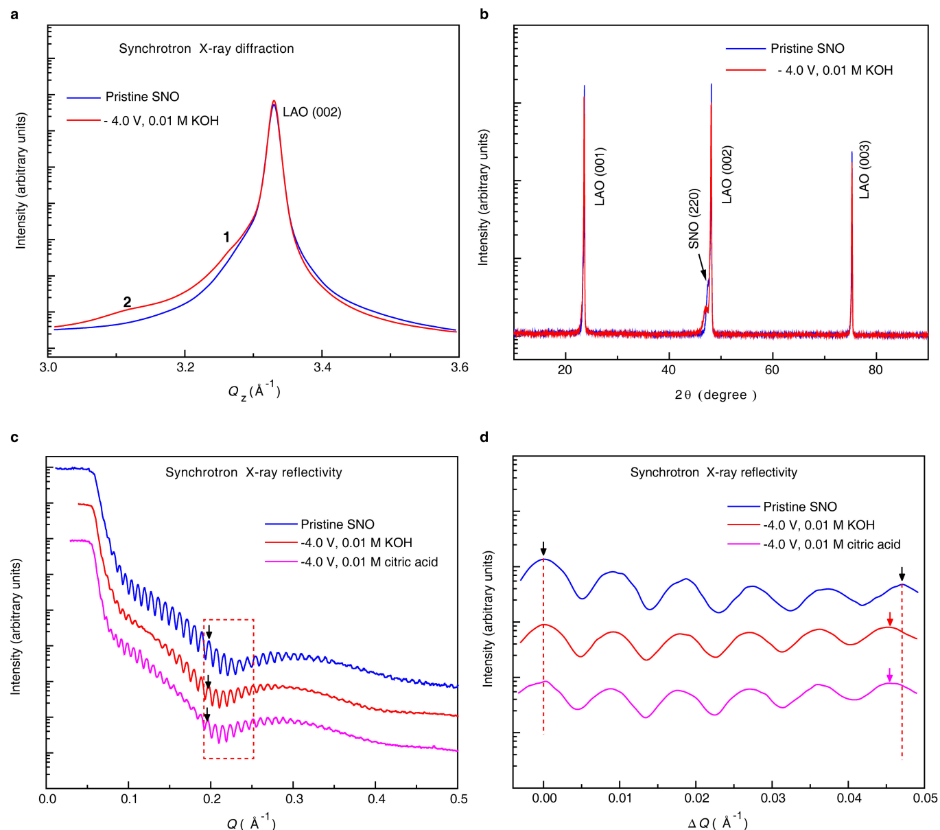
Extended Data Figure 6 | X-ray diffraction and X-ray reflectivity of water-treated SNO. a , Synchrotron X-ray diffraction curves taken from a SNO/LaAlO 3 thin film after treatment in a 0.01 M KOH aqueous solution at -4.0 V for 30 s. The (220) peak of pristine SNO (orthorhombic notation) appears at Q_1 \approx 3.29 \text{\AA}^{-1} as a shoulder with slightly lower scattering vector Q_z than the LaAlO 3 (002) diffraction peak (pseudocubic notation), demonstrating the epitaxial growth of SNO on LaAlO 3 . After the water treatment, the epitaxial relationship of SNO on LaAlO 3 is preserved. Peak 1 shifts to a lower Q_z . Peak 2 appears at Q_z = 3.11 \text{\AA}^{-1} , which corresponds to increase of the lattice constant by 5.7%. LAO stands for LaAlO 3 . b , X-ray diffraction profiles of SNO and water-treated SNO
